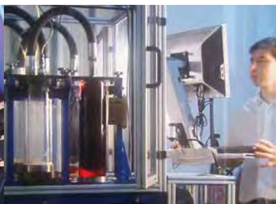
Bladder accumulator test bench - Patented technology
